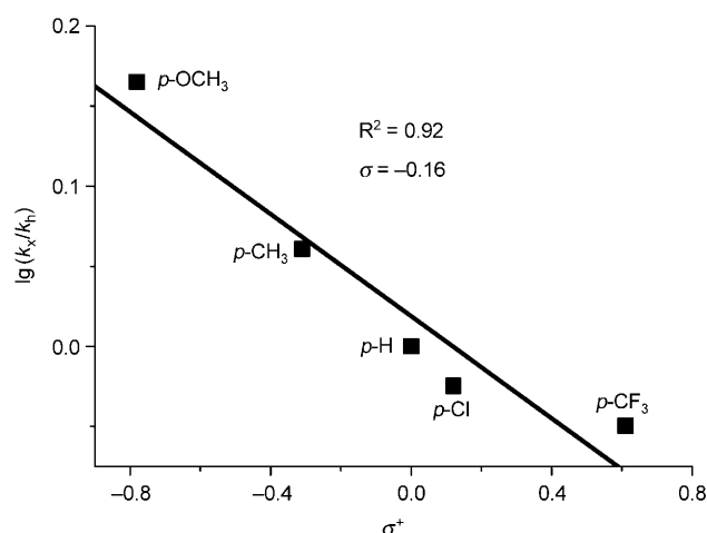
Figure 1. Hammett plots for the oxidation of substituted benzylamines with oxygen using mpg-C 3 N 4 catalyst. Hammett plots were obtained from a ratio of conversion with reaction time of 30 min.
